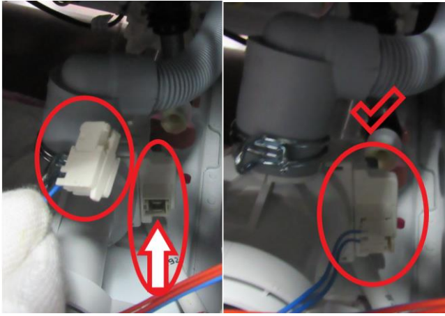
3.3. Connect the drain pump connector
