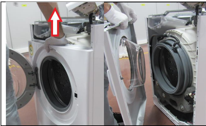
2.10. Pull up and remove the front panel.
