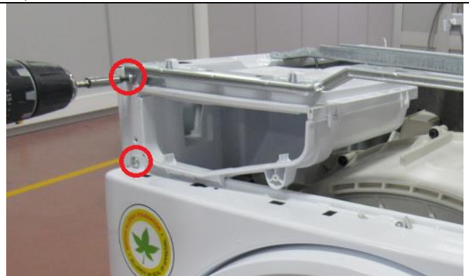
3.9. Tighten the screw on support bracket and two screws fixing front panel to body
